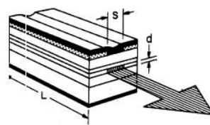
Traditional edge-emitter
