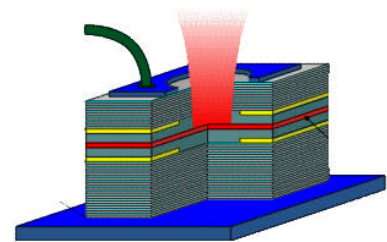
Novel surface-emitter
