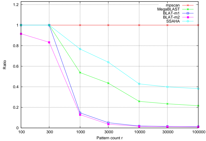
Fig. 6: Sensitivity of MEGABLAST, BLAT, and SSAHA compared to MPSCAN as the percentage of found matches after filtering. Influence of the number of tags on sensitivity (with l = 30 bp). The sensitivity of similarity search tools decreases strongly with the number of tags for short tags.
