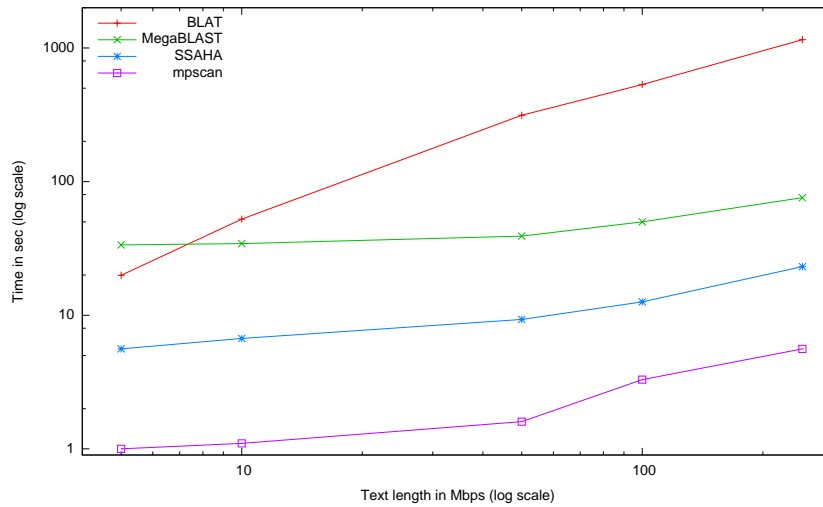
Fig. 5: Search times of BLAT, MEGABLAST, SSAHA, MPSCAN in seconds for 200 Kilo-patterns (LongSAGE tags of 21 bp), on increasing pieces of length 5, 10, 50, 100, and 247 Mbp of Human chromosome 1. Both axes have logarithmic scales. These curves illustrate the sublinear increase of time with respect to text length for all tools except BLAT, and the superiority of MPSCAN in running time.
