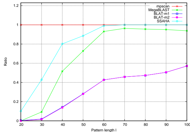
Fig. 4: Sensitivity of MEGABLAST, BLAT, and SSAHA compared to MPSCAN as the percentage of found matches after filtering. Influence of tag length on sensitivity (with r = 10,000 tags). Columns BLAT-m1 and BLAT-m2 allows to compare the sensitivity of BLAT when the filtration criterion asks for one or two seed matches, respectively; BLAT-m1 found necessarily more matches than BLAT-m2. However, here their curves are superimposed. The sensitivity of similarity search tools is low ( < 0.5 ) for tags \leq 30 bp and reaches a maximum for MEGABLAST and SSAHA at \geq 60 bp.
